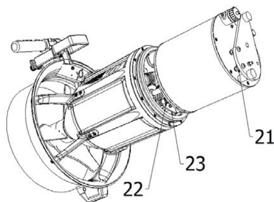
Figure 7 (view of the ADV without the external case)
